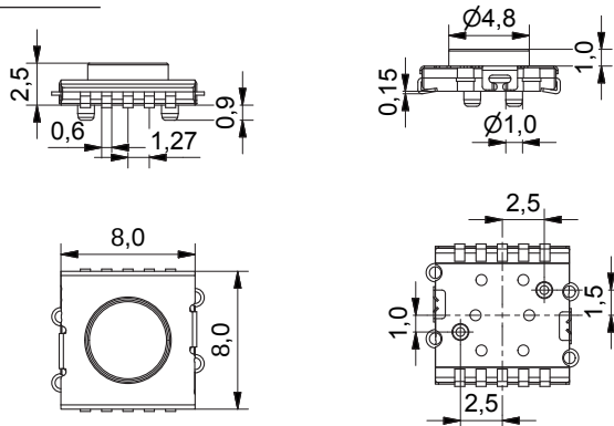
Switch 6C
